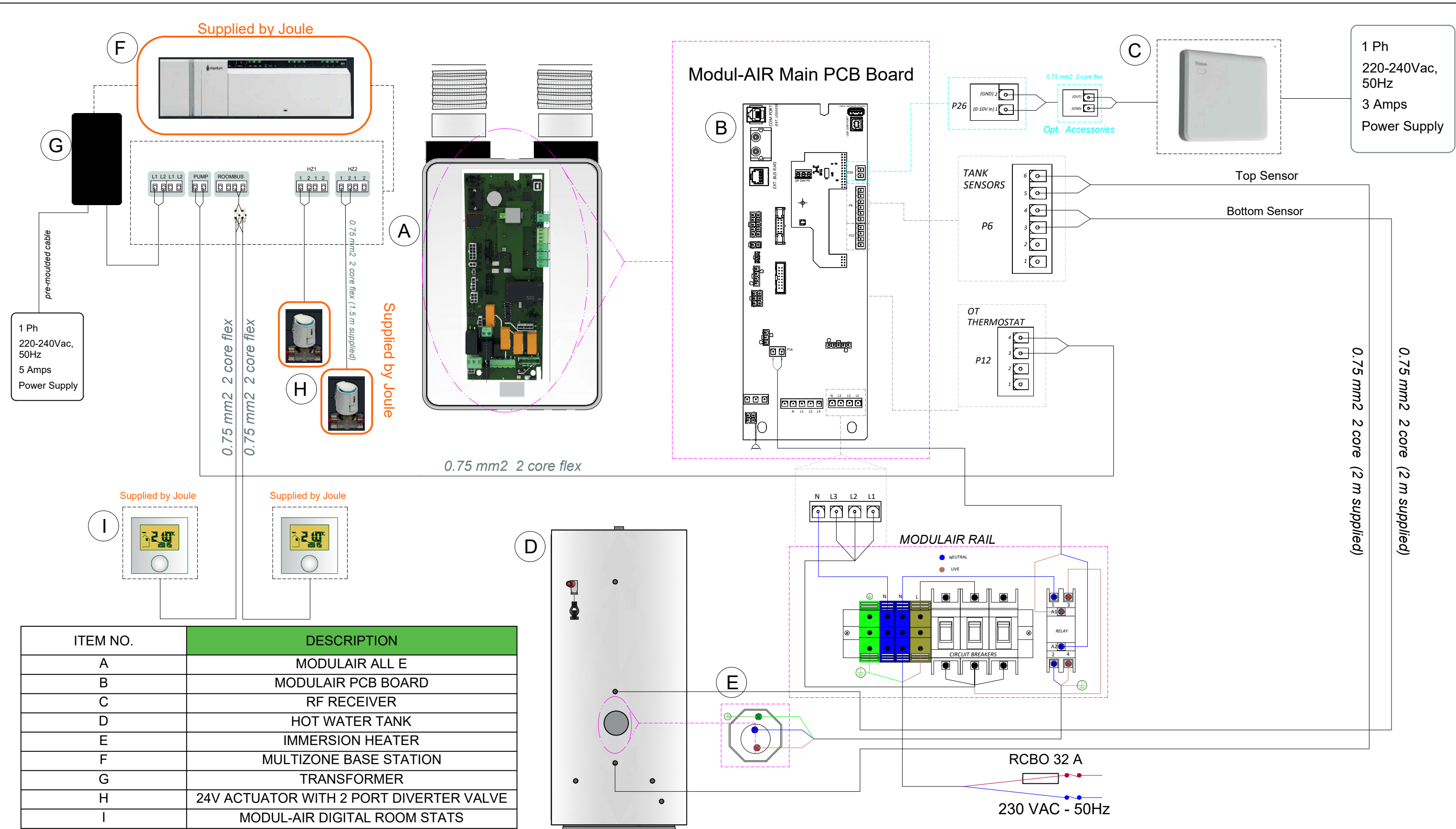
Modulair All-E with 2 Zone Radiators Electrical Schematic
