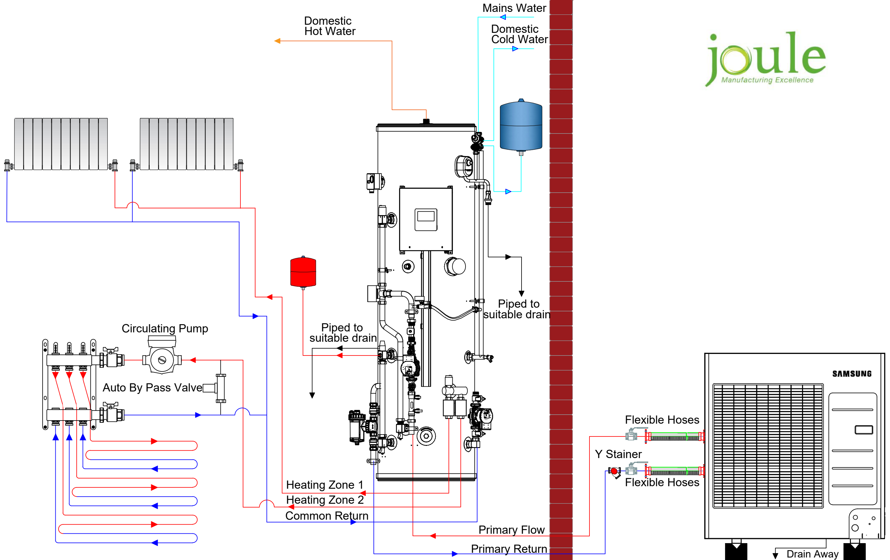
SAMSUNG ASHP WITH ZENITH DHW AND 2 HEATING ZONE 1x RADS & 1 x UFHs Front View of Unit & Cylinder
